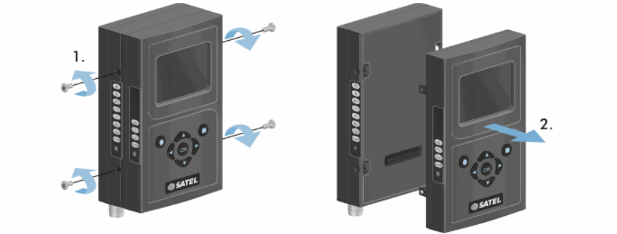
Figure 1.4 Modular construction, mounting of the central unit CU
