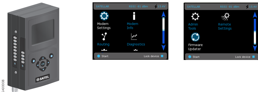
Figure 5.4 RU together with Central Unit (CU) equipped with LCD display and keypad, the main views
